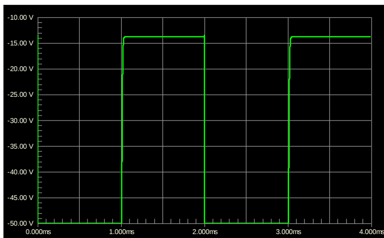
Figure 4.43 - Simulation of the shutter circuit in the program Circuit Maker, for 500 Hz square wave input signal, corresponding to 1 ms activation time.
