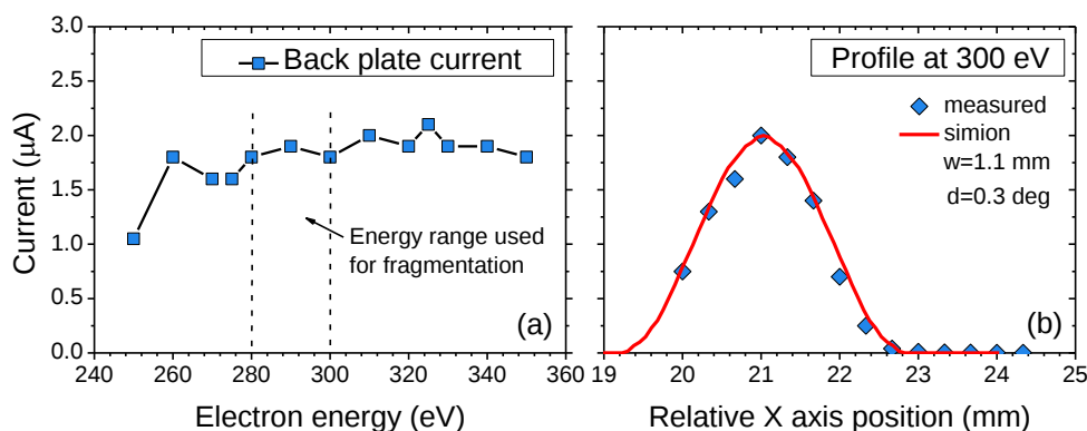
Figure 6.19 - Electron current measured at the back plate of the ion trap: a) plot of the back plate current versus the electron energy and b) electron beam profile. Simulated profile in SIMION is obtained for the beam width of 1.1 mm and pencil angle of 0.3 degrees and is in a good agreement with the measured profile.
