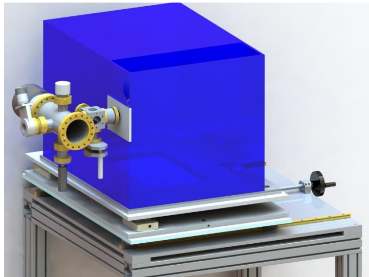
Figure 4.18 - 3D model of the vacuum stage coupled to the LTQ mass spectrometer, installed on an adjustable supporting frame, which is rested on a rigid table. Entire system is mobile. Designed by A. Milosavljević et al [9].
