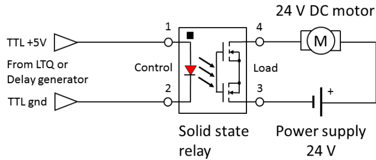
Figure 4.24 - Electrical circuit for the mechanical shutter. Solid state relay (SSR) switch consist of an IR photo-diode and two field effect transistors (FETs) with a photosensitive gate. High state of TTL signal turns on the photo-diode which results in a closing of the two transistors, closes the circuit on the right side by applying 24 V to the electric motor. Absence of TTL signal (or low state - 0 V) leads to the open circuit and electric motor is not powered.
