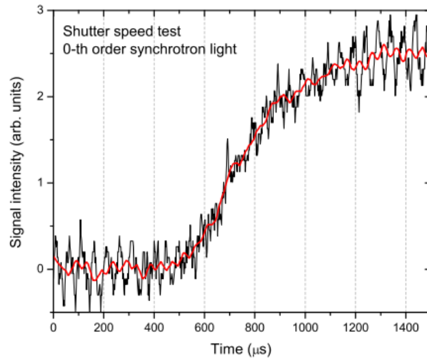
Figure 4.25 - Photodiode current generated by the zero-th order of synchrotron radiation light, measured after opening the mechanical shutter under high vacuum. Red line is generated by 50 point Savitzky Golay smoothing of the obtained signal, in order to reduce the noise. Adopted from [57].
