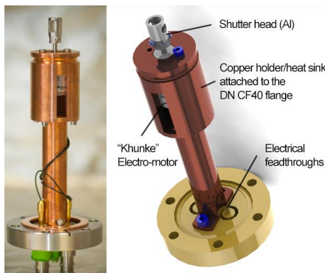
Figure 4.22 - Mechanical shutter for the chopping of photon beam. Picture of the shutter assembly mounted on a CF40 flange is on the left. 3D model of the shutter assembly is on the right. Adapted from [57].
