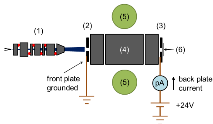
Figure 6.18 - Electrical scheme for the current measurement: 1) electron gun, 2) LTQ front plate - grounded, 3) LTQ back plate - connected to pico-ampere meter, 4) ion trap, 5) ion detectors and 6) aluminum foil attached to back plate.
