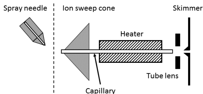
Figure 4.8 - Schematic representation of an API source of the LTQ XL mass spectrometer. Spray needle is a part of an independent detachable assembly - of the standard ESI or a nano-ESI source.
