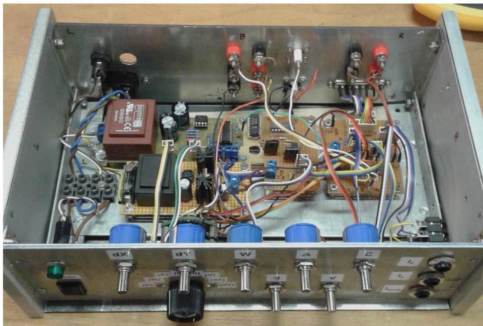
Figure 4.45 - Photograph of the electron gun power supply assembled for the present experiment. Electronic shutter circuit is integrated in the box. External high power supply for the cathode and high voltage supply which defines the electron energy are connected at the back side.
