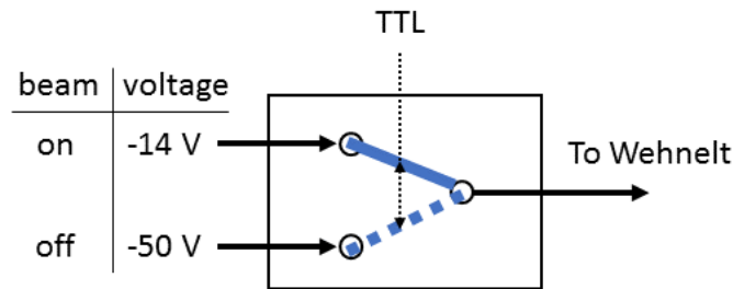
Figure 4.40 - Basic principle of operation of the electronic shutter circuit. In the upper position a switch connects -14 V to the W electrode, enabling the electron emission. Electron emission is completely blocked if the switch is in the lower position, where -50 V is applied to the W electrode.
