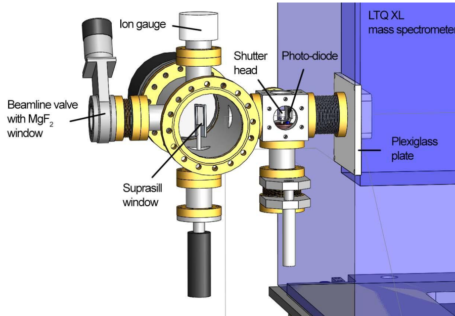
Figure 4.16 - 3D model of the differential turbo pumping assembly fitted with mechanical shutter, ion gauge, photodiode and a turbo pump. Designed by A. Milosavljević et al [9].
