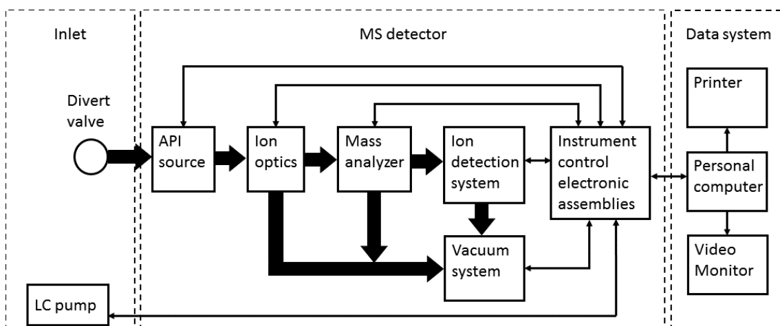
Figure 4.7 - Functional block diagram of LTQ XL mass spectrometer. Adopted from [47].
