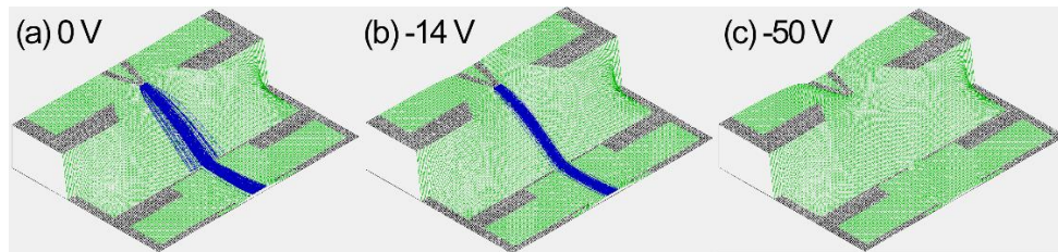
Figure 4.38 - Electric field and electron beam trace simulation from program SIMION. Voltages applied on Wehnelt electrode are relative to the cathode voltage: a) 0 V, b) -14 V and c) -50 V. High enough negative voltage completely blocks the electron emission.
